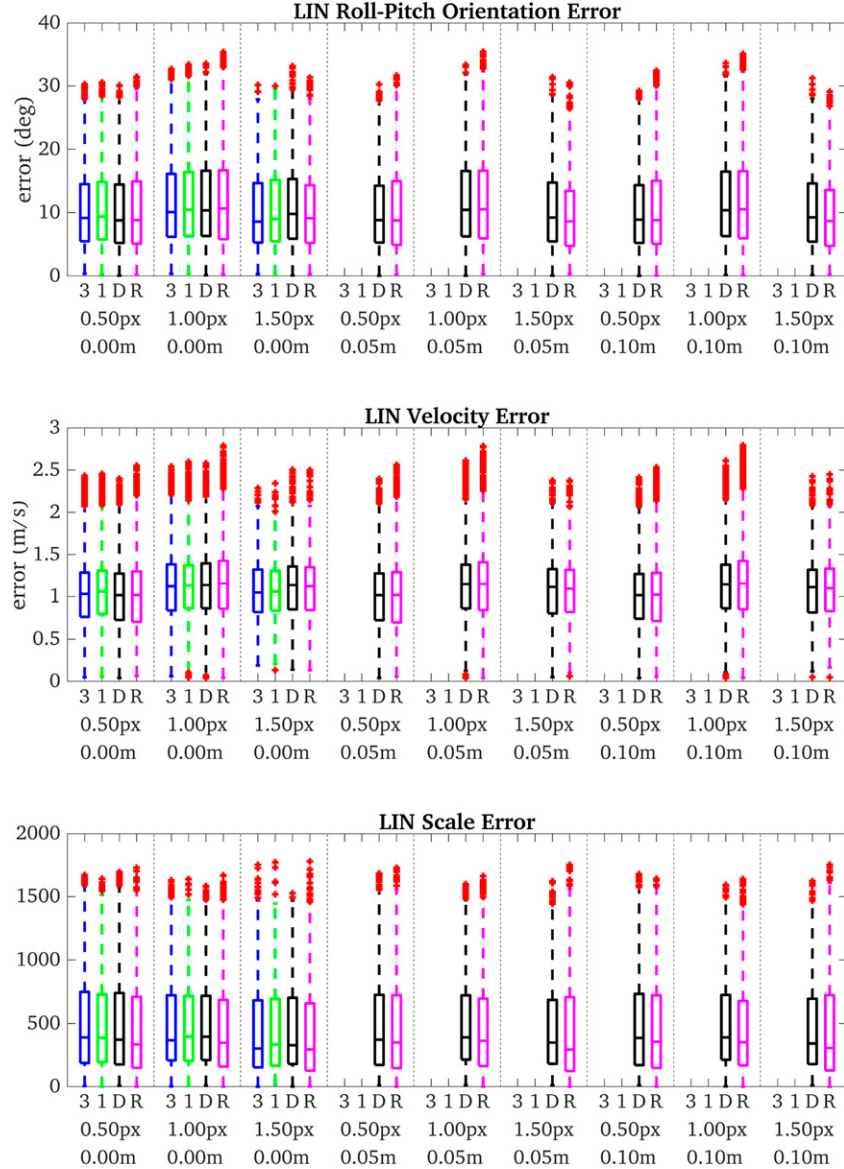
Figure 6. Orientation and velocity errors of the final pose of each linear system for different noise levels of feature bearings (px) and depths (m, on scaled depth pre-normalization). We define: DS 3D as 3 (blue), DS 1D as 1 (green), Ours w/o RANSAC as D (black), and Ours as R (magenta). Note that outliers outside the sample 3\sigma bound have been filtered for presentation clarity.
