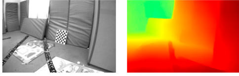
Figure 19. Qualitative result of the MiDaS Ranftl et al. (2022) v2.1 small on the EuRoC Vicron Room 1 sequence. The network can easily get confused about the unusual decor, such as on strips the floor.
